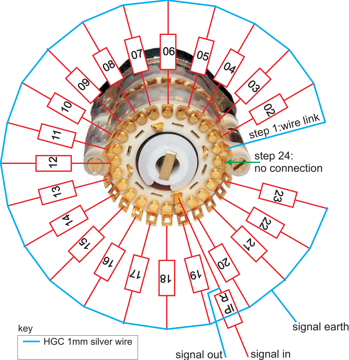
Fig 7. Shows the layout of one channel of the Shinkoh stepped attenuator
