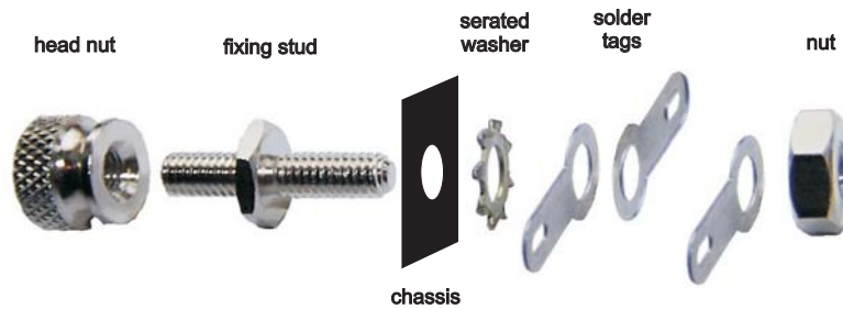
FIG. 2 exploded view of earth post composite parts
