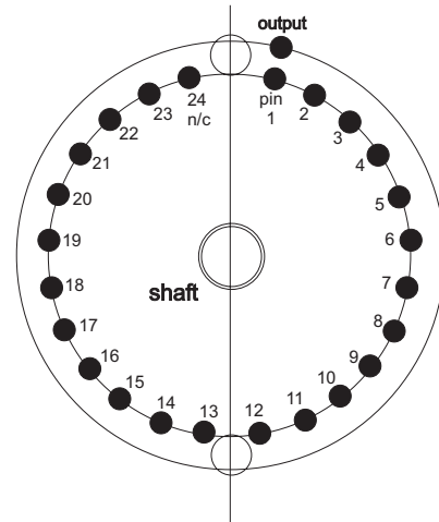
Diagram of one channel of the Dale 2 pole 23 way switch. Viewed from shaft end
