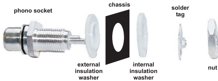
FIG. 1 exploded view of phono socket composite parts
