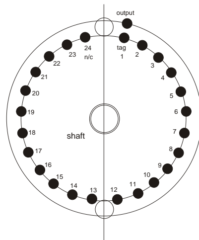
Diagram of one channel of the Dale 2 pole 23 way switch. Viewed from shaft end
